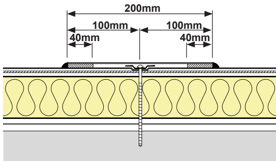
(fig 5 intermediate fixing)
