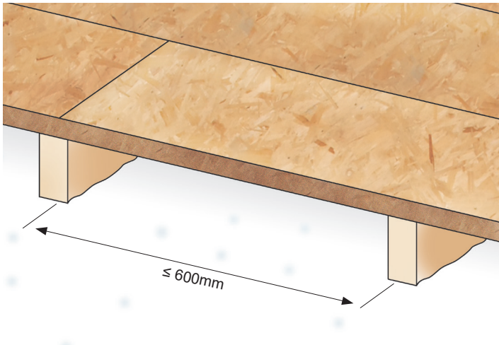
SMARTPLY LOFT Panels are suitable for joist centres up to 600mm in dry loft space
