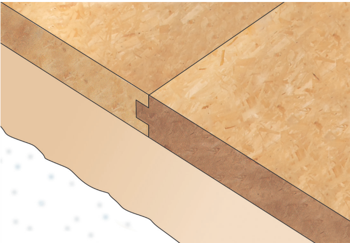
Install panels with expansion gap facing down
