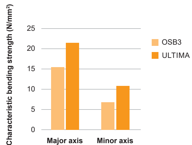
FIGURE 2: 35% increase in characteristic bending strength compared to OSB
